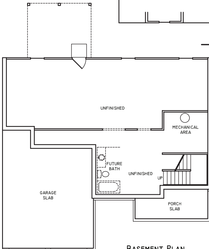
BASEMENT PLAN
