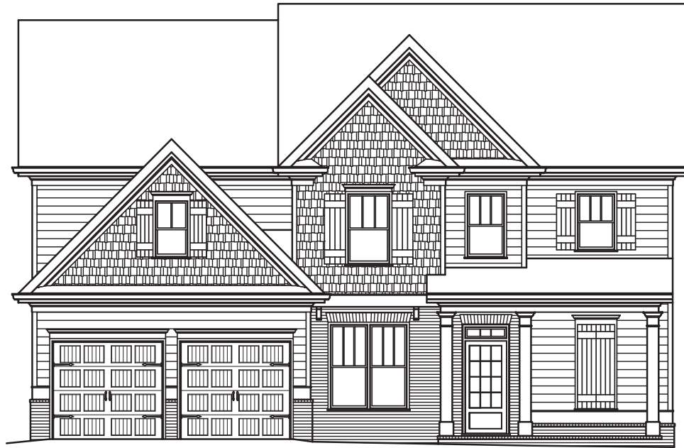
FRONT ELEVATION LOT 31 POD 3: GREAT SKY
