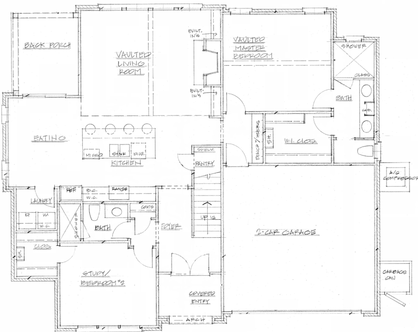
First Floor- 1519 sq. ft.
